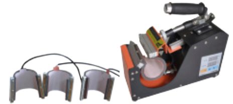
CM22-MGPRO4P Semi Automatic Mug Press with 4 mug pads
